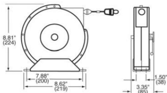
Dimensions static discharge reel
